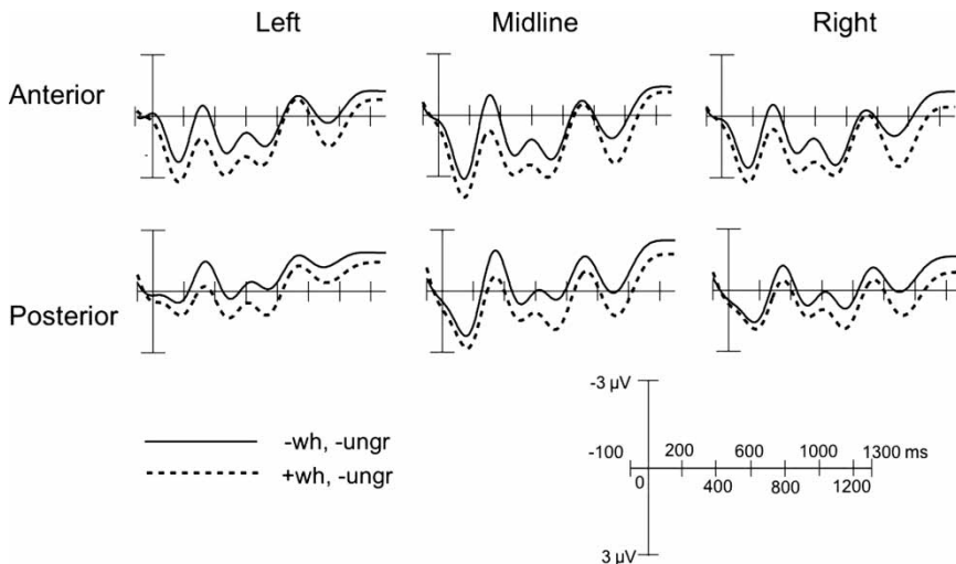
Figure 3. Grand average ERPs at six groups of topographically arranged electrode sites in the control and grammatical wh -dependency conditions (examples (a) and (c) in Table 1).
